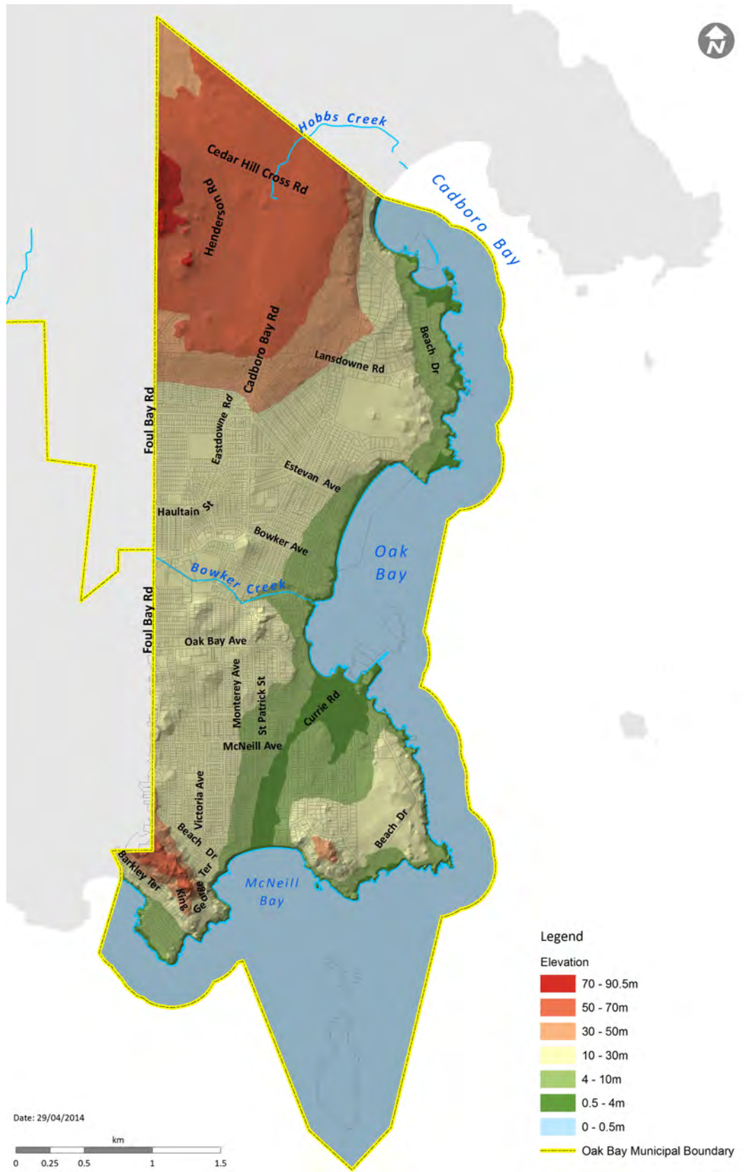
Figure 3.2: Elevation Map
